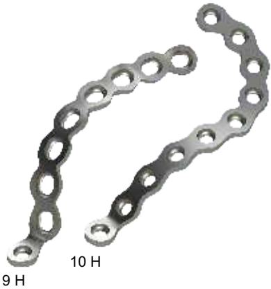
Posterior Wall Acetabular Plate with Ø 3,5 mm screw
