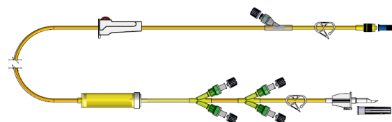
IV CHEMOTHERAPY INFUSION SET, 4-WAY CONNECTOR WITH CHECK-VALVE, NEEDLE-FREE Y-CONNECTION PORT, LIGHT-PROTECTED LARGE-BORE (3.0x4.1mm), 227cm DEHP-FREE TUBING
