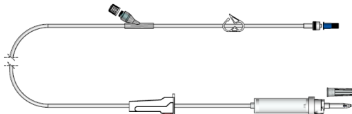
IV INFUSION SET, NEEDLE-FREE Y-CONNECTION PORT, TRANSPARENT LARGE-BORE (3.0x4.1mm), 235cm DEHP-FREE TUBING
